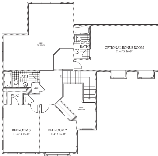
UPPER LEVEL FLOOR PLAN Bonus Room Option
